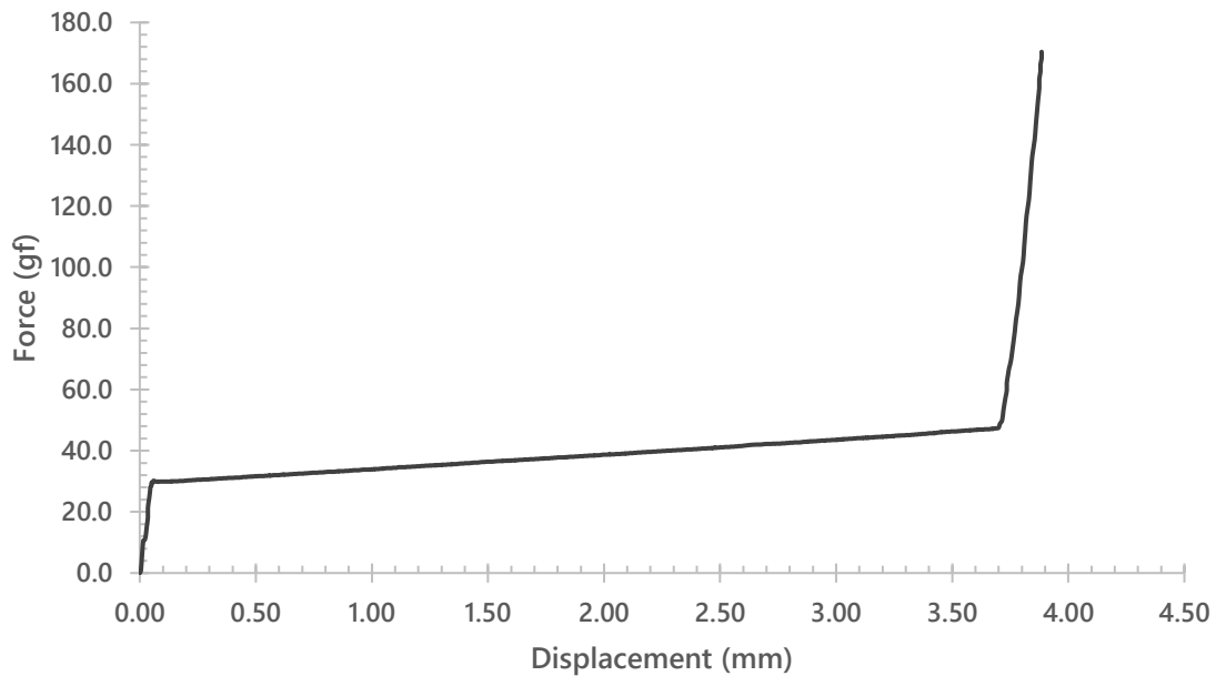
Everglide Sticky Rice Magnetic (Upstroke)
